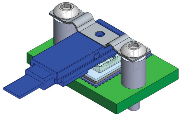
Figure 3: X80S Fury transceiver assembled onto PWB with RVCON™ cable attached
