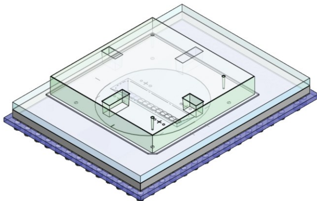
Figure 2: Top view of X80S Fury transceiver
